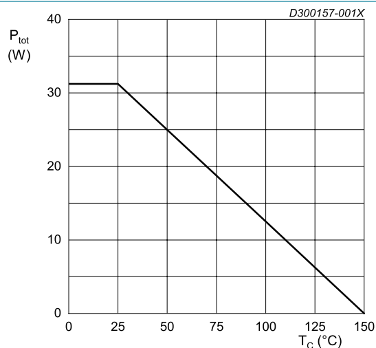
Fig. 1. Total power dissipation as a function of case temperature
