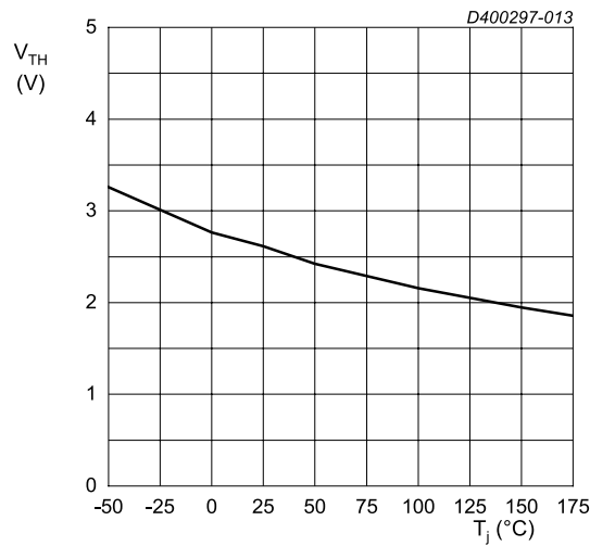
V_{DS} = V_{GS}; I_{DS} = 5\text{ mA} Fig. 13. Threshold voltage as a function of junction temperature
