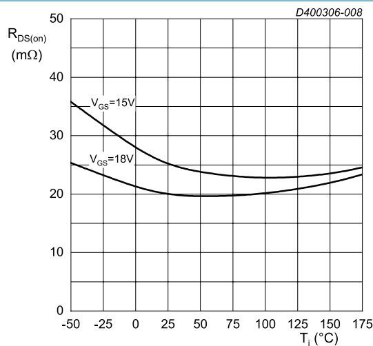
I_{DS} = 45\text{ A} ; t_p < 200\text{ }\mu\text{s} Fig. 8. Drain-source on-state resistance as a function of junction temperature
