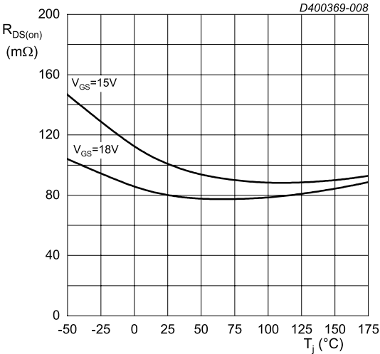
I_{DS} = 10\text{ A} ; t_p < 200\text{ }\mu\text{s} Fig. 8. Drain-source on-state resistance as a function of junction temperature
