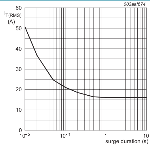
f = 50 Hz; T_{mb} = 126 °C Fig. 3. RMS on-state current as a function of surge duration; maximum values
