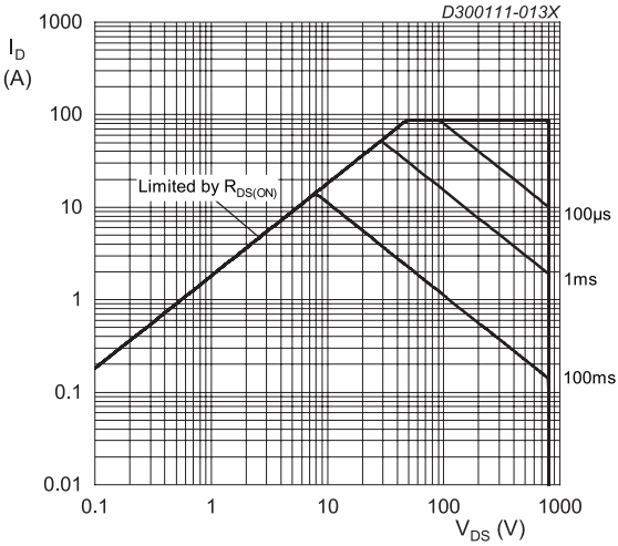
T_h = 25\text{ }^{\circ}\text{C} Fig. 13. Safe operating area
