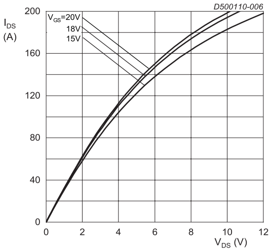
Fig. 6. Output characteristics; drain current as a function of drain-source voltage; typical values T_j = 150\text{ °C}; t_p < 200\ \mu\text{s}
