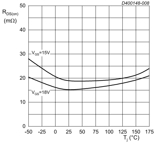
I_{DS} = 55 A; t_p < 200 \mu s Fig. 8. Drain-source on-state resistance as a function of junction temperature
