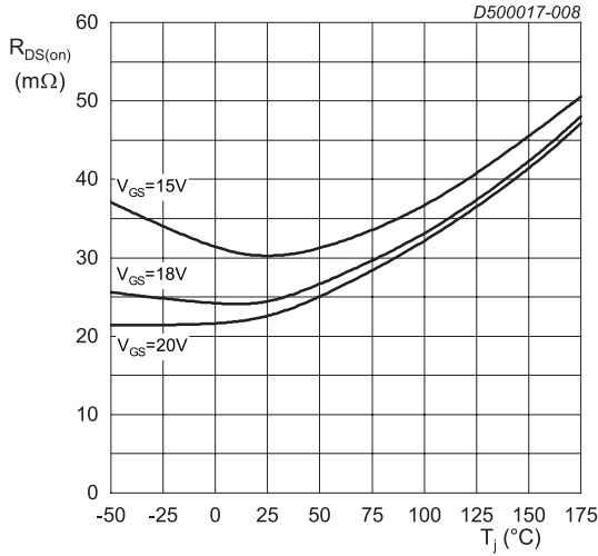
I_{DS} = 40 \text{ A}; t_p < 200 \mu\text{s} Fig. 8. Drain-source on-state resistance as a function of junction temperature
