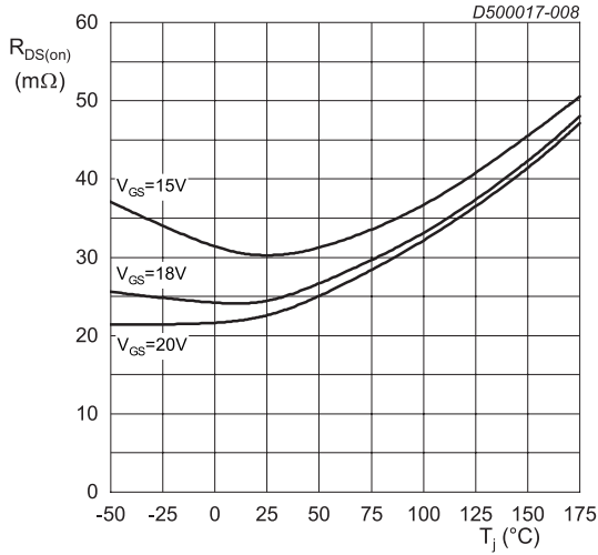
I_{DS} = 40 A; t_p < 200 \mu s Fig. 8. Drain-source on-state resistance as a function of junction temperature
