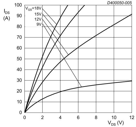
Fig. 5. Output characteristics; drain current as a function of drain-source voltage; typical values T_j = 25\text{ }^\circ\text{C}; t_p < 200\text{ }\mu\text{s}
