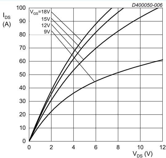
Fig. 6. Output characteristics; drain current as a function of drain-source voltage; typical values T_j = 175\text{ }^\circ\text{C}; t_p < 200\text{ }\mu\text{s}
