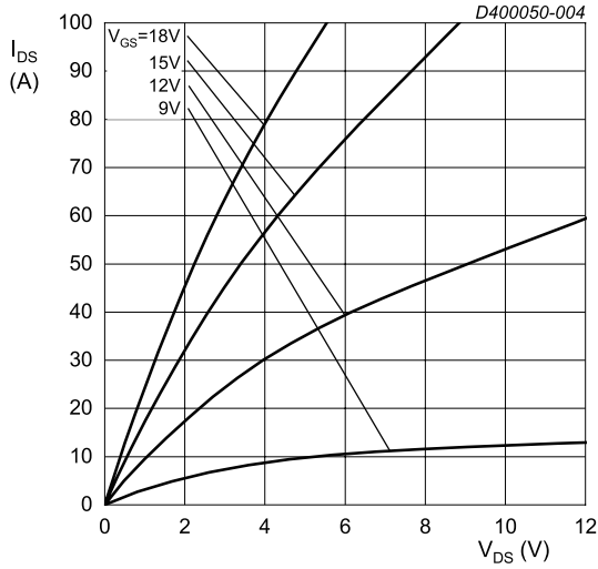
Fig. 4. Output characteristics; drain current as a function of drain-source voltage; typical values T_j = -55\text{ }^\circ\text{C}; t_p < 200\text{ }\mu\text{s}
