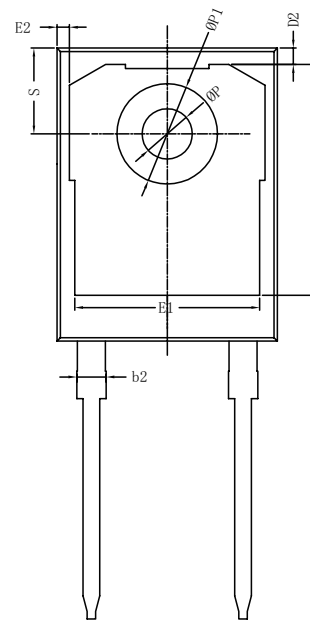
BOTTOM VIEW
