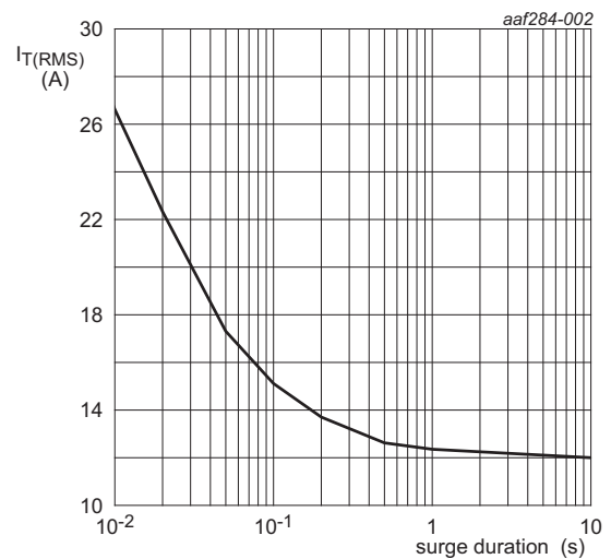
Fig. 2. RMS on-state current as a function of surge duration; maximum values f = 50 Hz; T_{\text{mb}} = 118\text{ °C}
