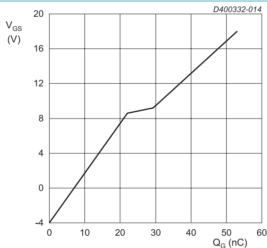
I_{DS} = 15\text{ A} ; I_{GS} = 0.1\text{ mA} ; V_{DS} = 400\text{ V} ; T_j = 25\text{ }^{\circ}\text{C} Fig. 14. Gate-source voltage as a function of gate charge; typical values
