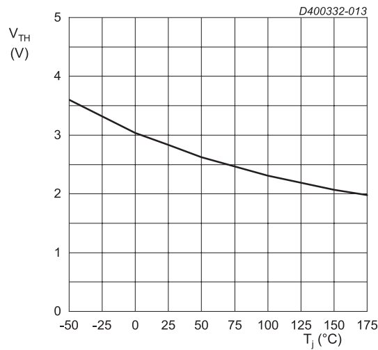
V_{DS} = V_{GS} ; I_{DS} = 4\text{ mA} Fig. 13. Threshold voltage as a function of junction temperature
