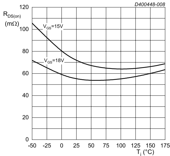
I_{DS} = 15\text{ A} ; t_p < 200\text{ }\mu\text{s} Fig. 8. Drain-source on-state resistance as a function of junction temperature
