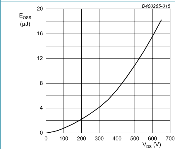
Fig. 15. Output capacitor stored energy as a function of drain-source voltage
