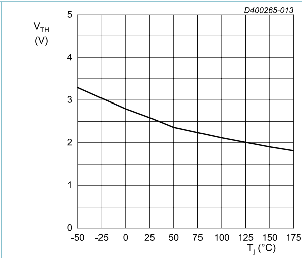
V_{DS} = V_{GS}; I_{DS} = 3.5\text{ mA} Fig. 13. Threshold voltage as a function of junction temperature
