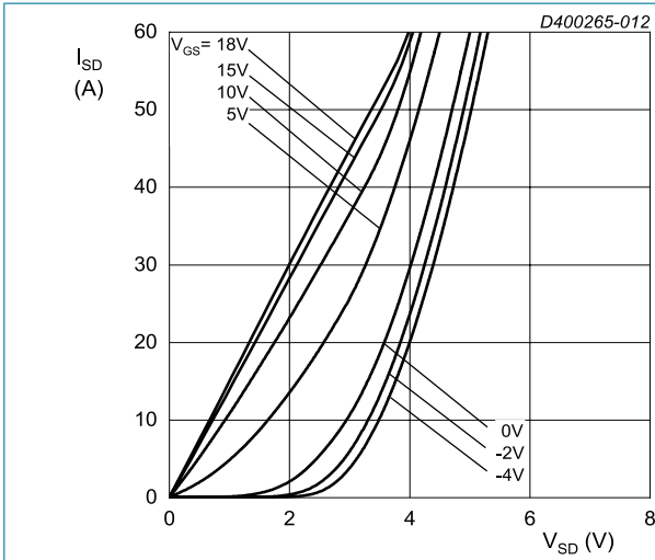
T_j = 175\text{ }^\circ\text{C}; t_p < 200\text{ }\mu\text{s} Fig. 12. Body diode forward characteristics; typical values
