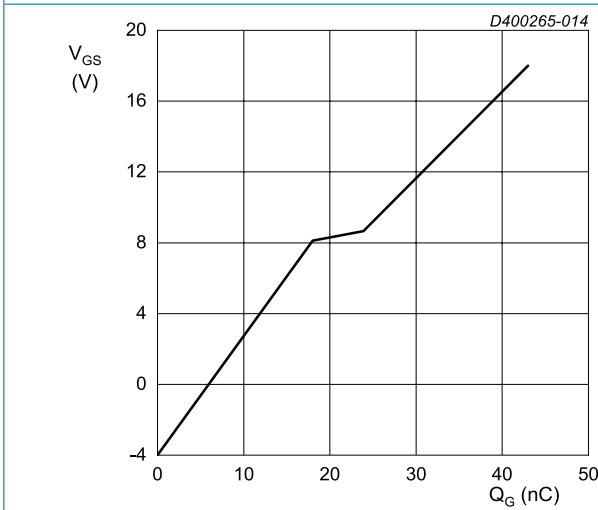
I_{DS} = 13\text{ A}; I_{GS} = 0.1\text{ mA}; V_{DS} = 400\text{ V}; T_j = 25\text{ }^\circ\text{C} Fig. 14. Gate-source voltage as a function of gate charge; typical values
