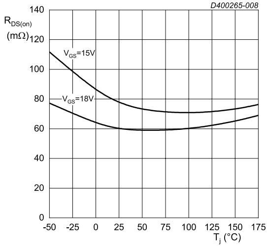
I_{DS} = 13 \text{ A}; t_p < 200 \mu\text{s} Fig. 8. Drain-source on-state resistance as a function of junction temperature
