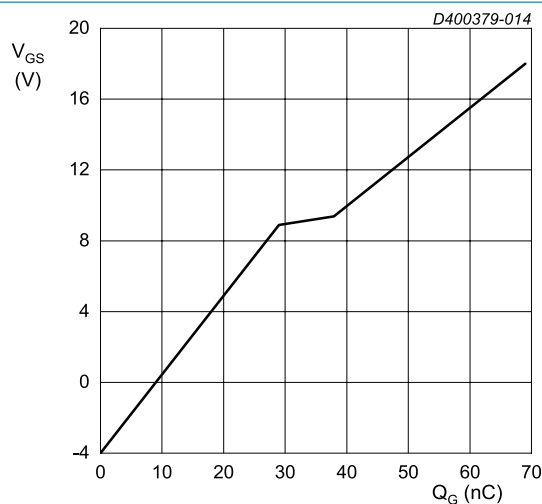
I_{DS} = 20\text{ A} ; I_{GS} = 0.1\text{ mA} ; V_{DS} = 400\text{ V} ; T_j = 25\text{ }^{\circ}\text{C} Fig. 14. Gate-source voltage as a function of gate charge; typical values
