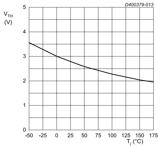
V_{DS} = V_{GS} ; I_{DS} = 5.5\text{ mA} Fig. 13. Threshold voltage as a function of junction temperature
