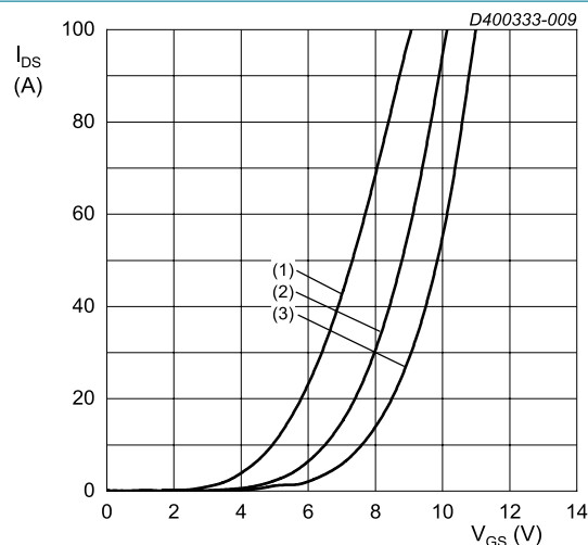
V_{DS} = 20\text{ V} ; t_p < 200\text{ }\mu\text{s} (1) T_j = 175^{\circ}C (2) T_j = 25^{\circ}C (3) T_j = -55^{\circ}C Fig. 9. Transfer characteristics; drain current as a function of gate-source voltage; typical values
