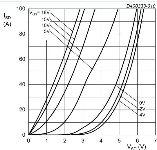
T_j = -55^{\circ}C ; t_p < 200\text{ }\mu\text{s} Fig. 10. Body diode forward characteristics; typical values
