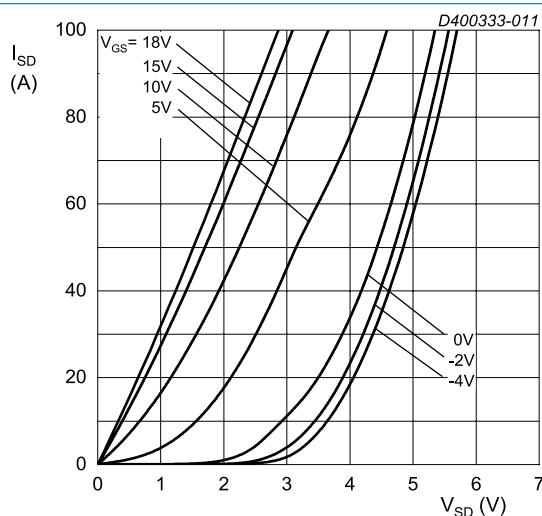
T_j = 25^{\circ}C ; t_p < 200\text{ }\mu\text{s} Fig. 11. Body diode forward characteristics; typical values
