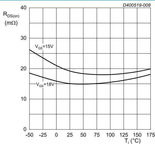
I_{DS} = 55\text{ A}; t_p < 200\text{ }\mu\text{s} Fig. 8. Drain-source on-state resistance as a function of junction temperature
