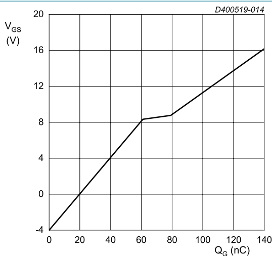
I_{DS} = 55\text{ A} ; I_{GS} = 0.1\text{ mA} ; V_{DS} = 400\text{ V} ; T_j = 25\text{ }^{\circ}\text{C} Fig. 14. Gate-source voltage as a function of gate charge; typical values
