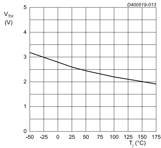
V_{DS} = V_{GS} ; I_{DS} = 14\text{ mA} Fig. 13. Threshold voltage as a function of junction temperature
