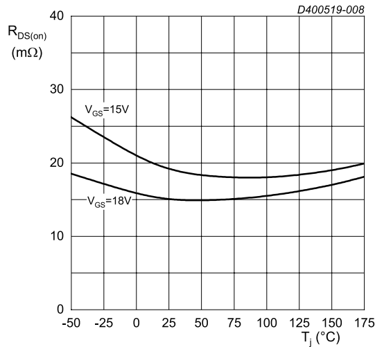
I_{DS} = 55\text{ A}; t_p < 200\text{ }\mu\text{s} Fig. 8. Drain-source on-state resistance as a function of junction temperature
