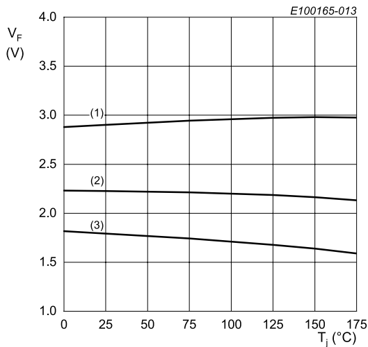
(1) I F = 50 A (2) I F = 25 A (3) I F = 12.5 A Fig. 13. Typical diode forward voltage as a function of junction temperature
