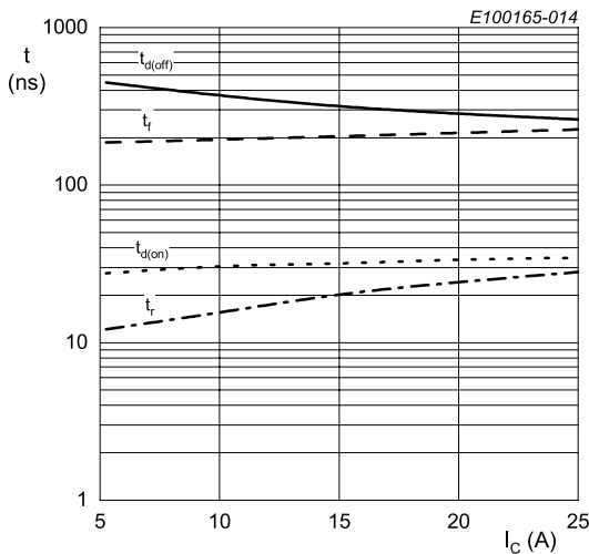
R g = 10 Ω; V GE = 15V/0V; T j = 175 °C; V CE = 600 V; inductive load Fig. 14. Typical switching times as a function of collector current
