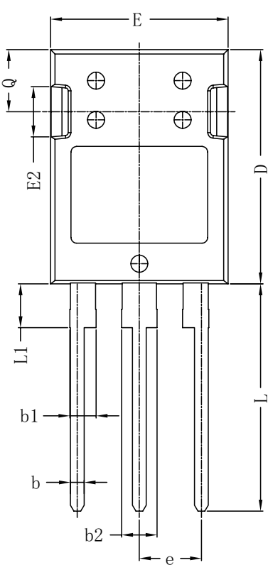
TOP VIEW
