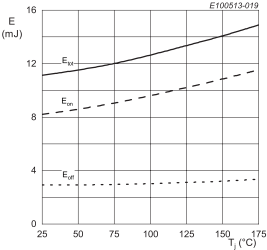
I_C = 160\text{ A} ; V_{GE} = 15\text{V}/-5\text{V} ; R_g = 3.6\ \Omega ; V_{CE} = 400\text{ V} ; inductive load Fig. 19. Typical switching energy losses as a function of junction temperature
