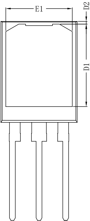
BOTTOM VIEW
