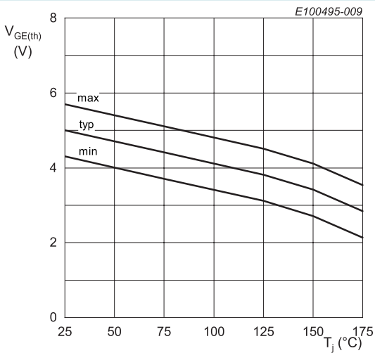
I_C = 1200 µA Fig. 9. Gate-emitter threshold voltage as a function of junction temperature
