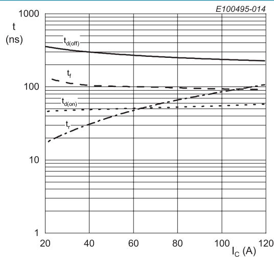
R_g = 3.6\ \Omega ; V_{GE} = 15\text{V}/-5\text{V} ; T_j = 175\text{ }^\circ\text{C} ; V_{CE} = 400\text{ V} ; inductive load Fig. 14. Typical switching times as a function of collector current
