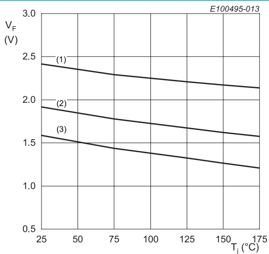
(1) I_F = 240\text{ A} (2) I_F = 120\text{ A} (3) I_F = 60\text{ A} Fig. 13. Typical diode forward voltage as a function of junction temperature
