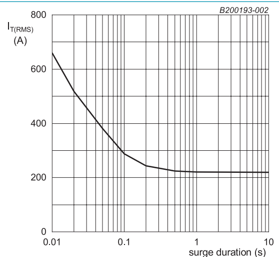
Fig. 2. RMS on-state current as a function of surge duration; maximum values f = 50\text{ Hz} ; T_{mb} = 90\text{ °C}
