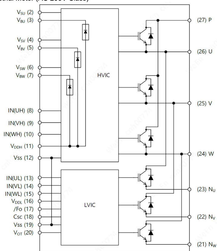
Figure 1. Internal Circuit
