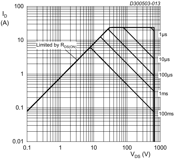
Fig. 13. Safe operating area T_C = 25\text{ }^{\circ}\text{C}
