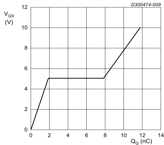
I_D = 3.5\text{ A}; V_{DS} = 400\text{ V} Fig. 9. Gate-source voltage as a function of gate charge; typical values
