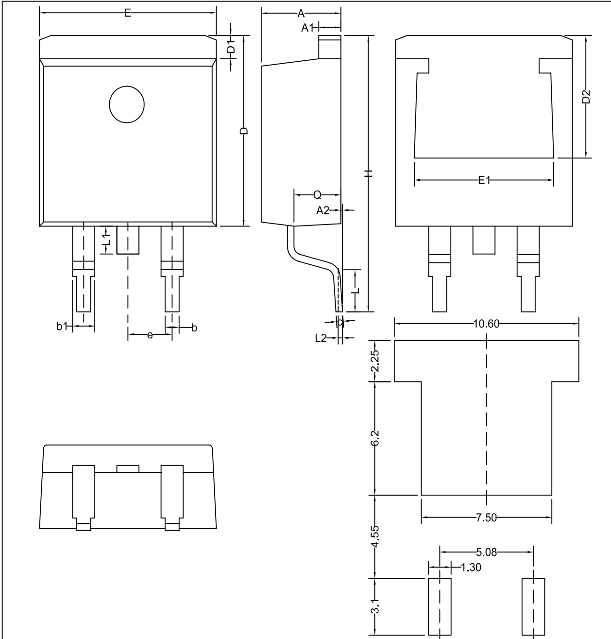
Recommended Footprint
