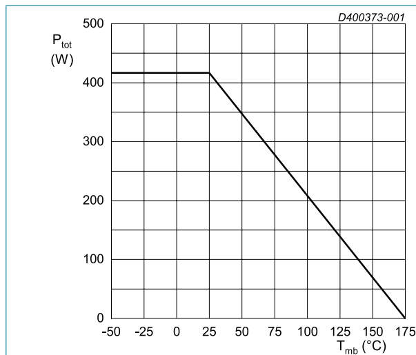
Fig. 1. Total power dissipation as a function of mounting base temperature; maximum values
