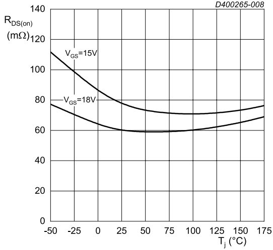
I_{DS} = 13 A; t_p < 200 \mu s Fig. 8. Drain-source on-state resistance as a function of junction temperature
