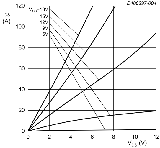
Fig. 4. Output characteristics; drain current as a function of drain-source voltage; typical values T_j = -55\text{ }^\circ\text{C}; t_p < 200\text{ }\mu\text{s}
