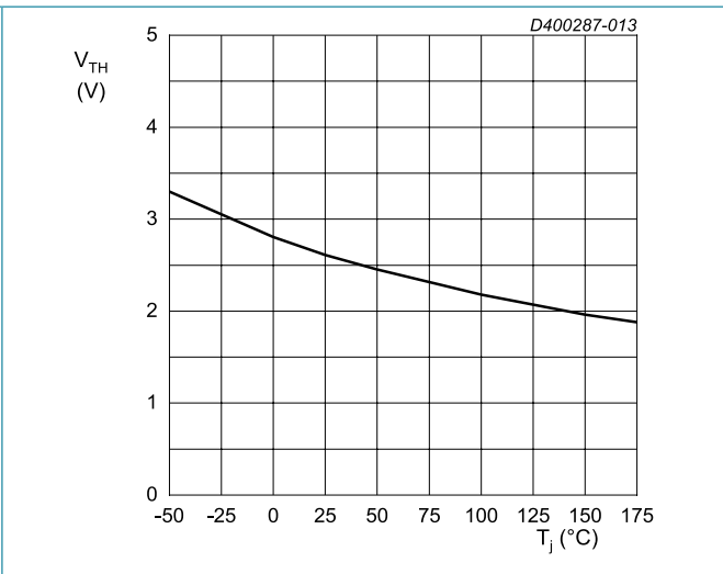
V_{DS} = V_{GS} ; I_{DS} = 6\text{ mA} Fig. 13. Threshold voltage as a function of junction temperature
