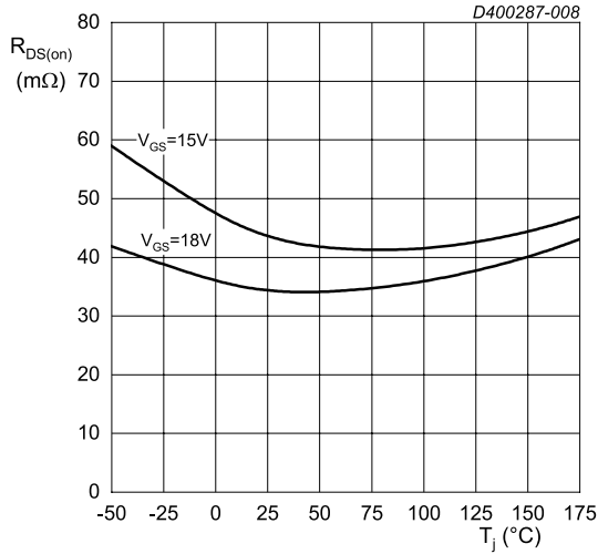
I_{DS} = 25 \text{ A}; t_p < 200 \mu\text{s} Fig. 8. Drain-source on-state resistance as a function of junction temperature
