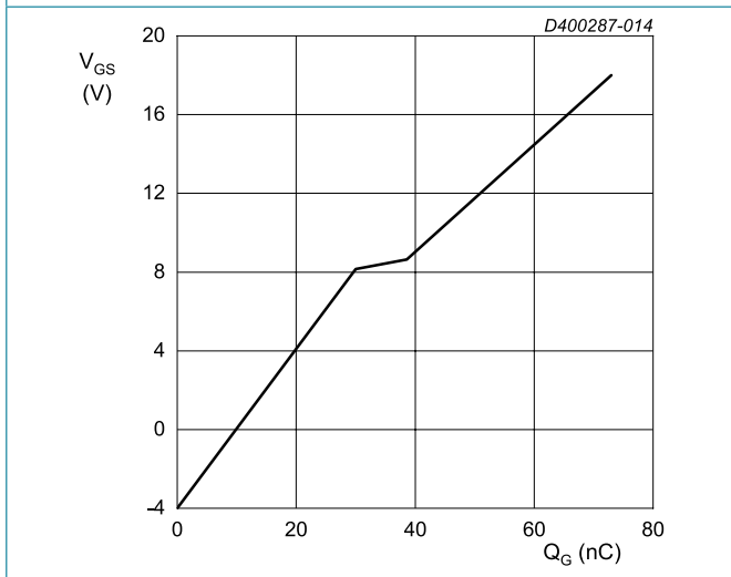
I_{DS} = 25\text{ A} ; I_{GS} = 0.1\text{ mA} ; V_{DS} = 400\text{ V} ; T_j = 25\text{ }^\circ\text{C} Fig. 14. Gate-source voltage as a function of gate charge; typical values
