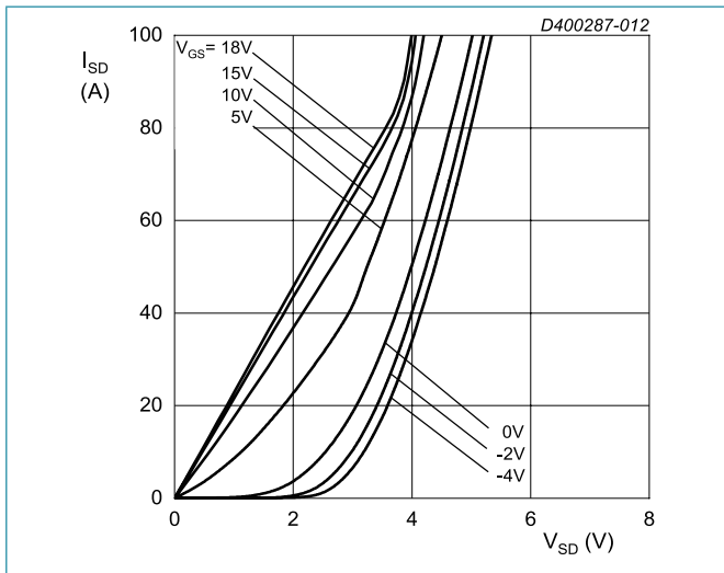
T_j = 175\text{ }^\circ\text{C} ; t_p < 200\text{ }\mu\text{s} Fig. 12. Body diode forward characteristics; typical values
