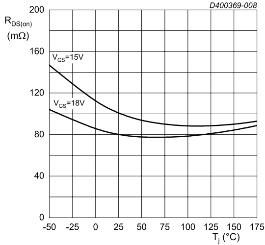
I_{DS} = 10 A; t_p < 200 \mu s Fig. 8. Drain-source on-state resistance as a function of junction temperature
