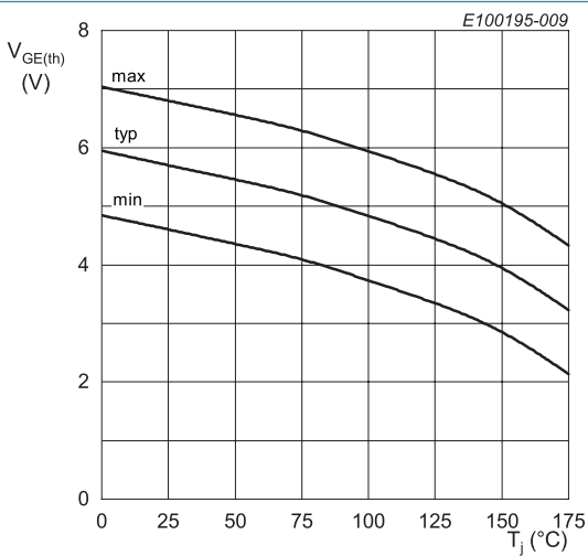
I_C = 500\text{ }\mu\text{A} Fig. 9. Gate-emitter threshold voltage as a function of junction temperature
