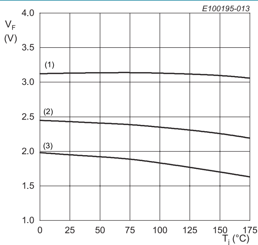
(1) I_F = 150\text{ A} (2) I_F = 75\text{ A} (3) I_F = 37.5\text{ A} Fig. 13. Typical diode forward voltage as a function of junction temperature
