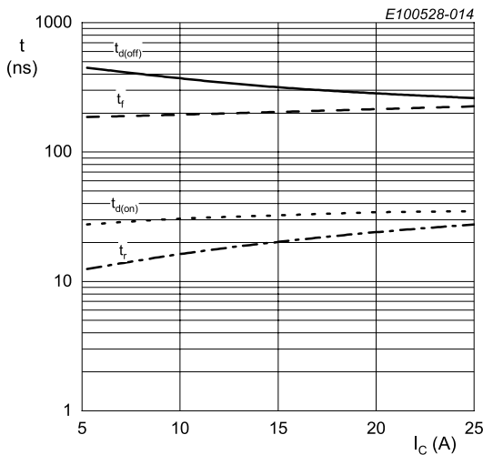
R_g = 10\ \Omega; V_{GE} = 15\text{V}/0\text{V}; T_j = 175\text{ }^\circ\text{C}; V_{CE} = 600\text{ V}; inductive load Fig. 14. Typical switching times as a function of collector current
