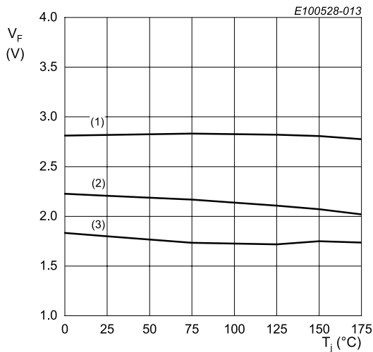
(1) I_F = 24\text{ A} (2) I_F = 12\text{ A} (3) I_F = 6\text{ A} Fig. 13. Typical diode forward voltage as a function of junction temperature
