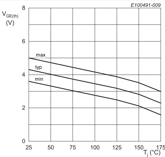
I_C = 1200\text{ }\mu\text{A} Fig. 9. Gate-emitter threshold voltage as a function of junction temperature
