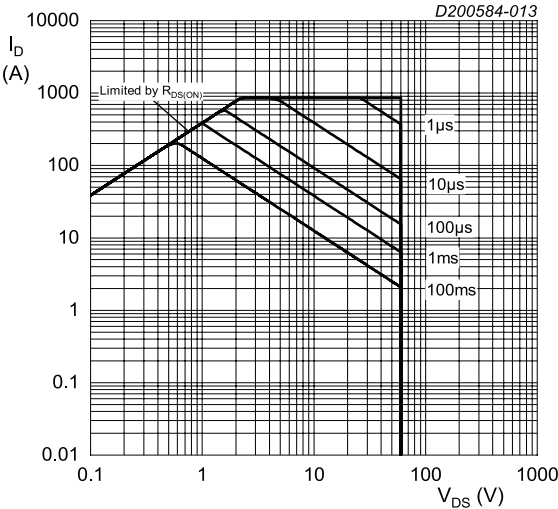
T_C = 25^\circ\text{C} Fig. 13. Safe operating area
