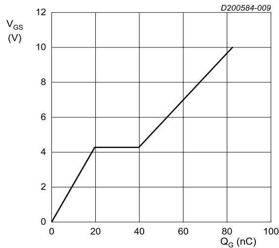
I_D = 20\text{ A}; V_{DS} = 30\text{ V} Fig. 9. Gate-source voltage as a function of gate charge; typical values
