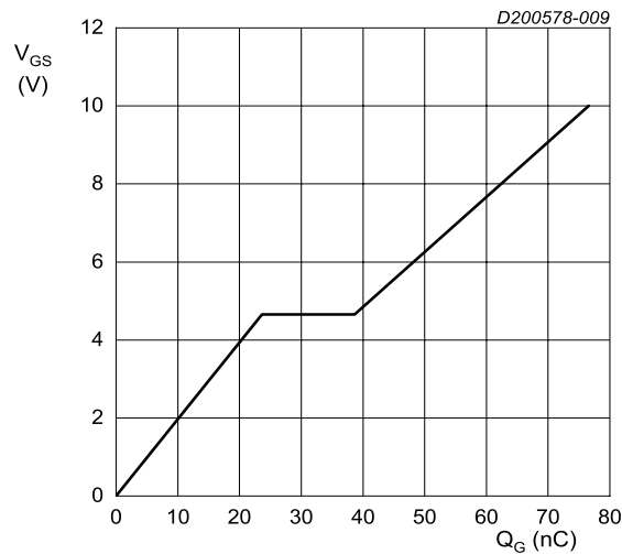
I_D = 20\text{ A}; V_{DS} = 20\text{ V} Fig. 9. Gate-source voltage as a function of gate charge; typical values
