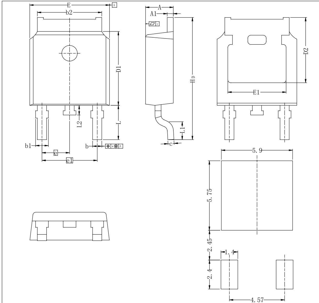
Recommended Footprint
