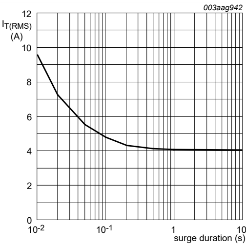
Fig. 2. RMS on-state current as a function of surge duration; maximum values f = 50\text{ Hz} ; T_{mb} = 108\text{ }^{\circ}\text{C}
