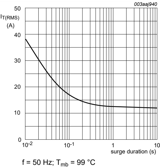
Fig. 2. RMS on-state current as a function of surge duration; maximum values f = 50\text{ Hz} ; T_{\text{mb}} = 99\text{ }^{\circ}\text{C}
