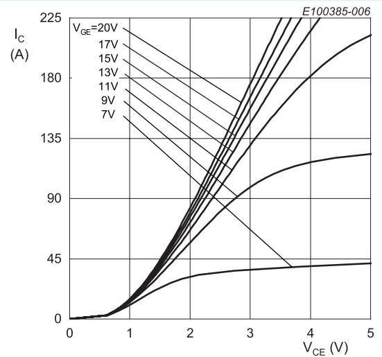
T_j = 175^\circ\text{C} Fig. 6. Typical output characteristic
