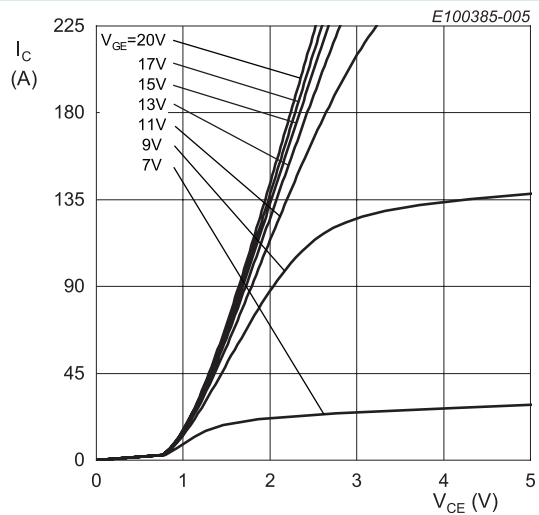
T_j = 25^\circ\text{C} Fig. 5. Typical output characteristic
