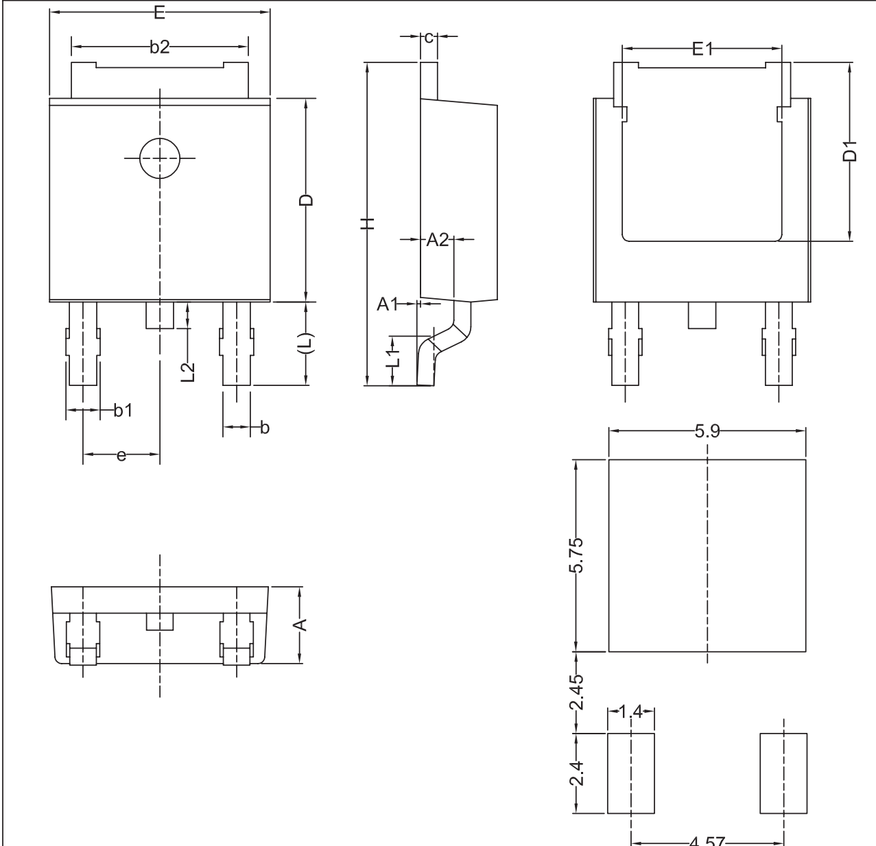
Recommended Footprint
