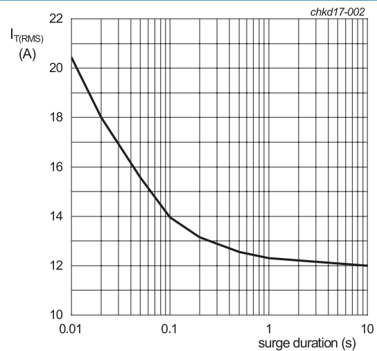
Fig. 2. RMS on-state current as a function of surge duration; maximum values f = 50\text{ Hz} ; T_{mb} = 123\text{ }^{\circ}\text{C}
